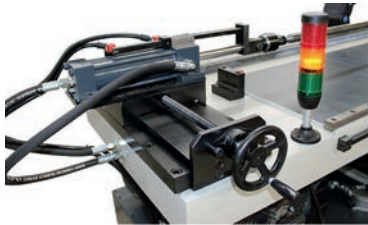
hydraulic mandrel
