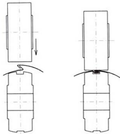
PIC: SKETCH PRESSING POSITION
